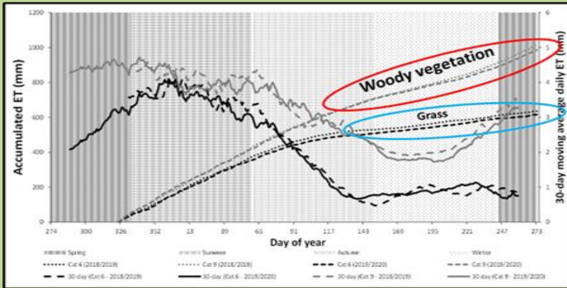
Figure 4.4 Measured total evaporation over a grassland catchment (Catchment 6, black lines) and a woody encroached catchment (Catchment 9, grey lines)
